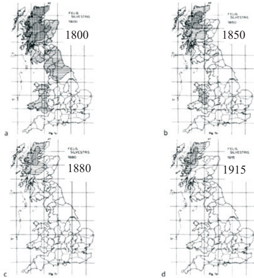
Fig. 2.1. Distribution of the wildcat in Great Britain in a) 1800, b) 1850, c) 1880 and d) 1915. Cross-hatching indicates common or widely distributed, horizontal shading indicates rare, declining or localised. White areas indicate extinct or data lacking, extinction presumed (Langley & Yalden 1977).
